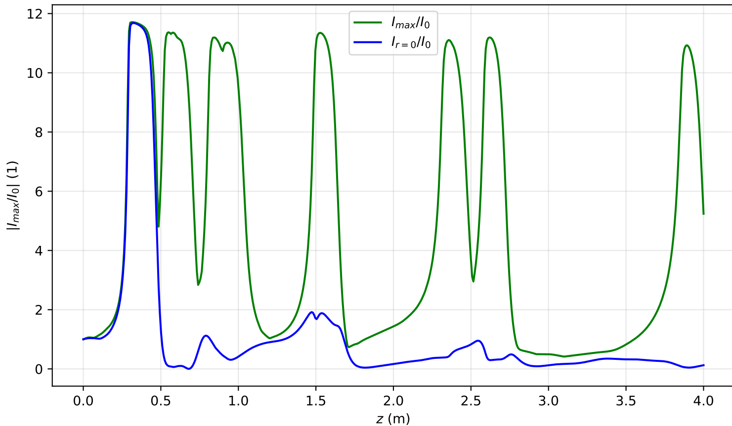
I_{max}(x=0, y=0, z)/I_0 , Pin=9.5Pcr, noisy input, artificial time
